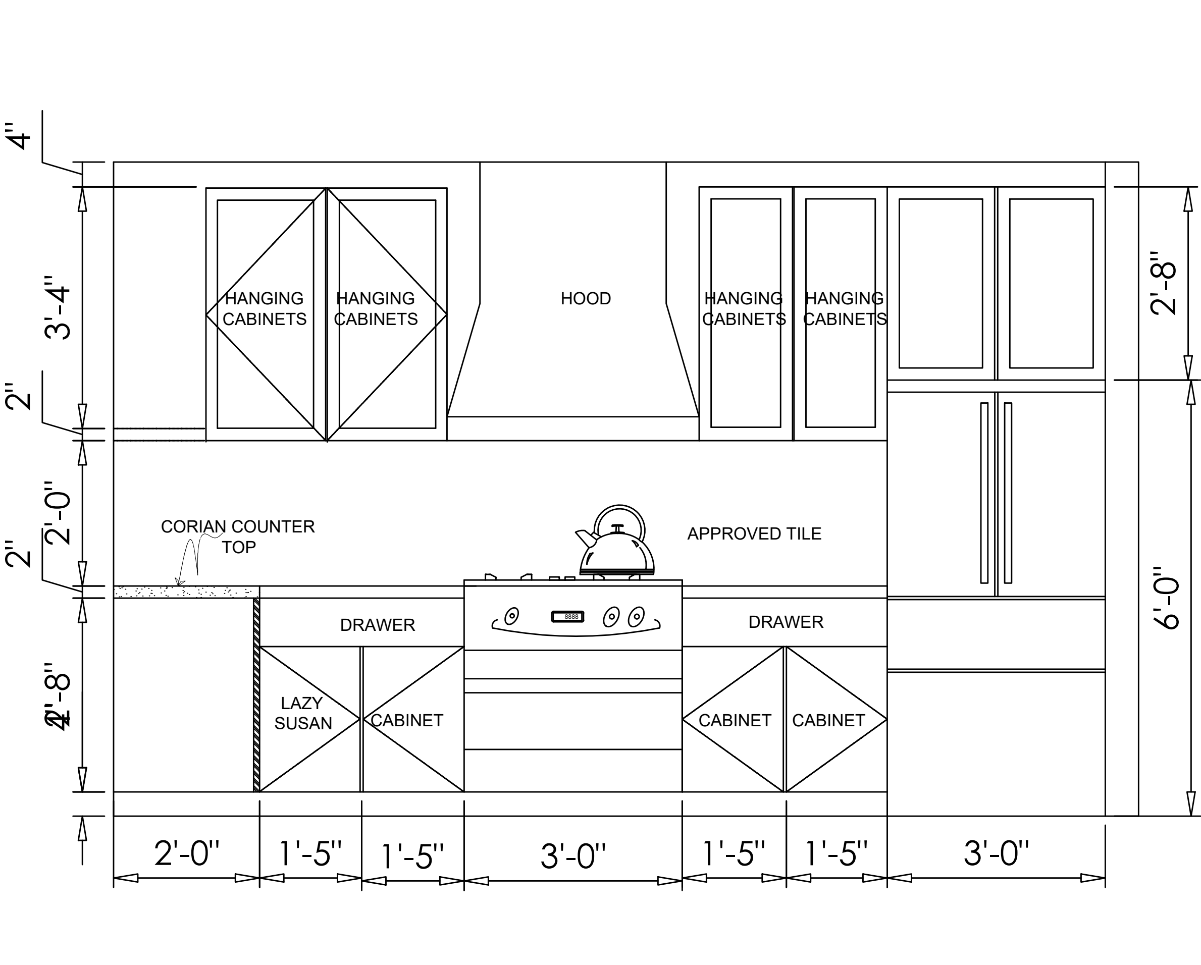
KITCHEN ELEVATION 1 SCALE : \frac{3}{4} " = 1'
