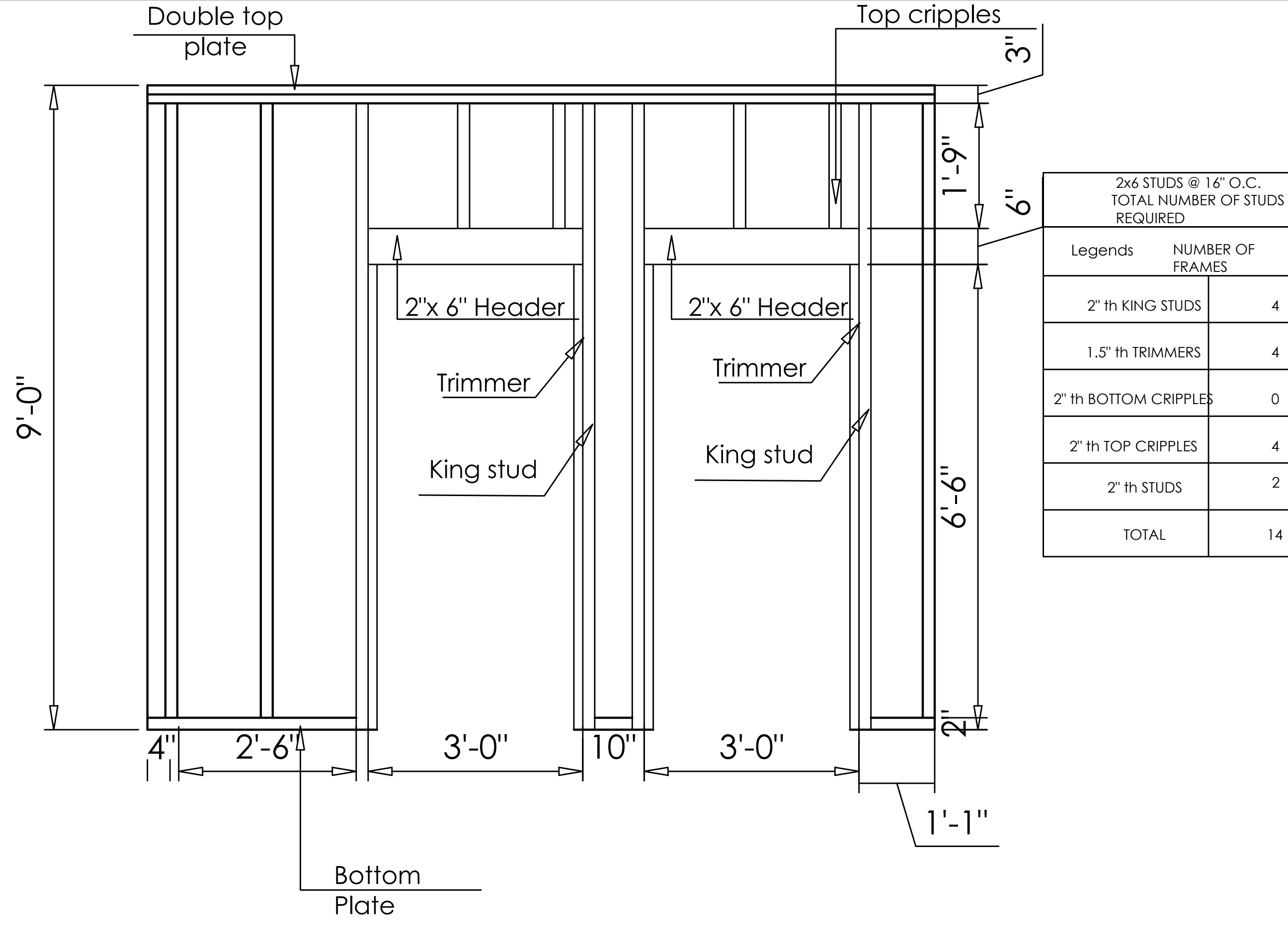
WALL E FRAMING DETAILS
