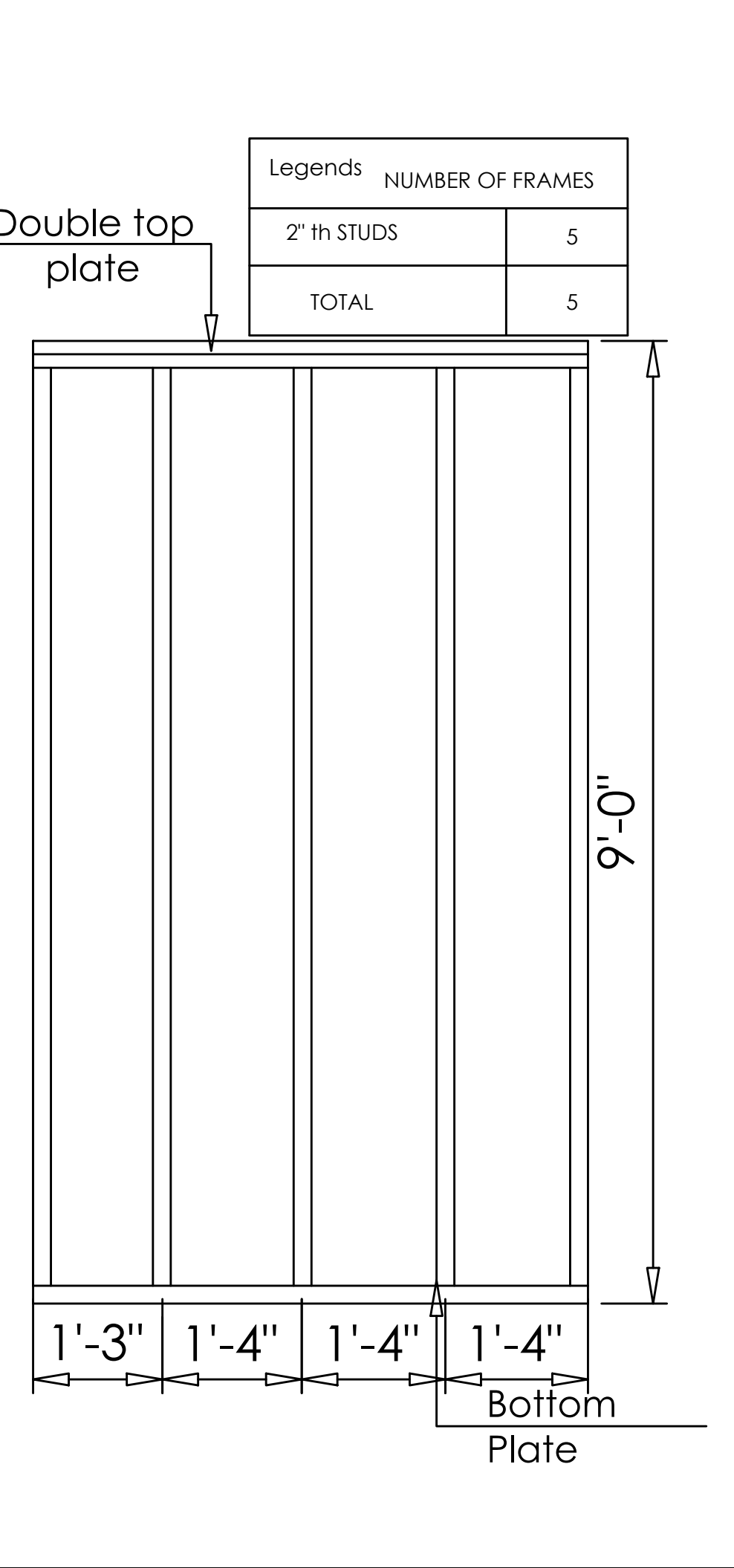
WALL F FRAMING DETAILS
