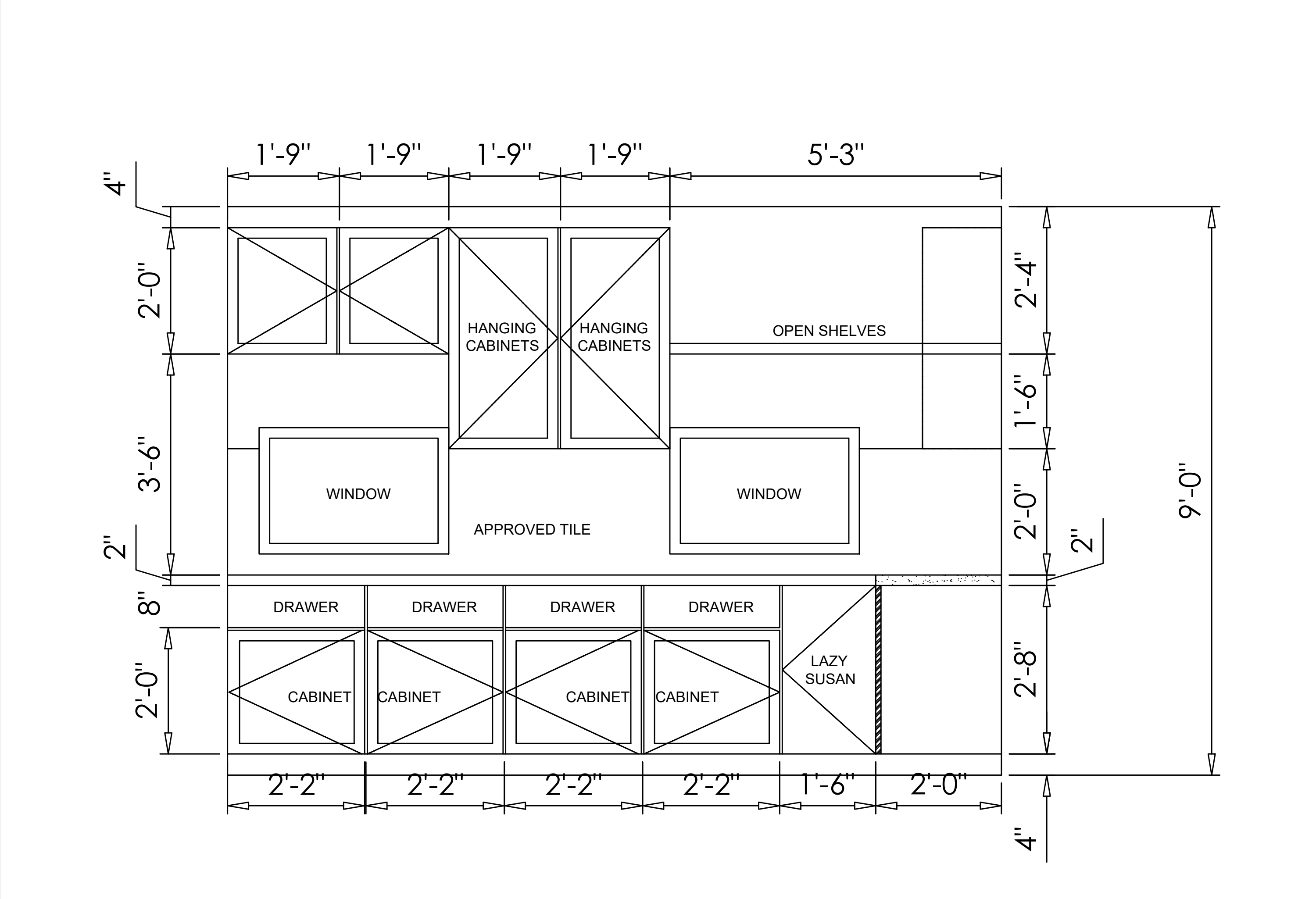
KITCHEN ELEVATION 3 SCALE : \frac{3}{4} " = 1'
