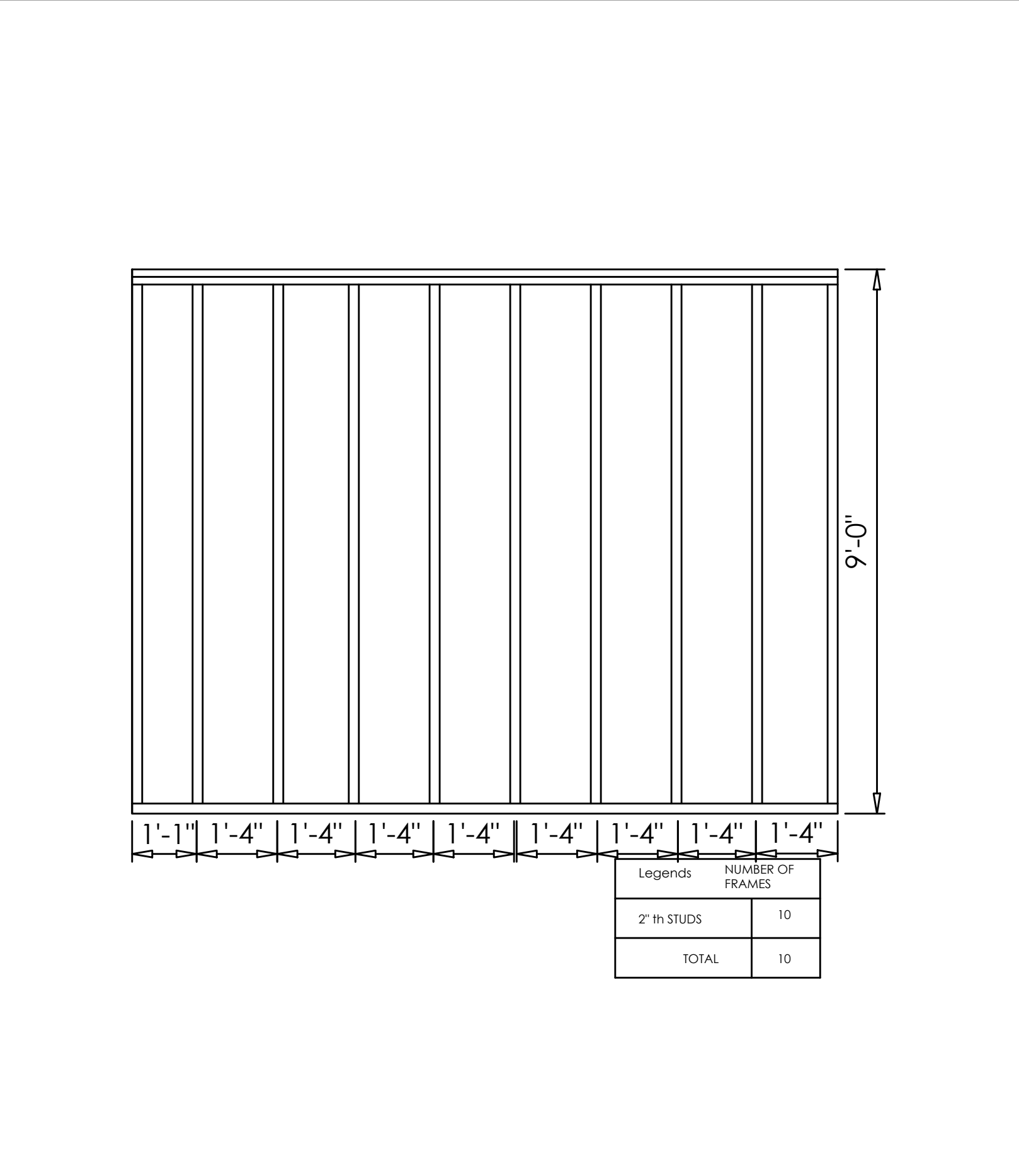
WALL G FRAMING DETAILS
