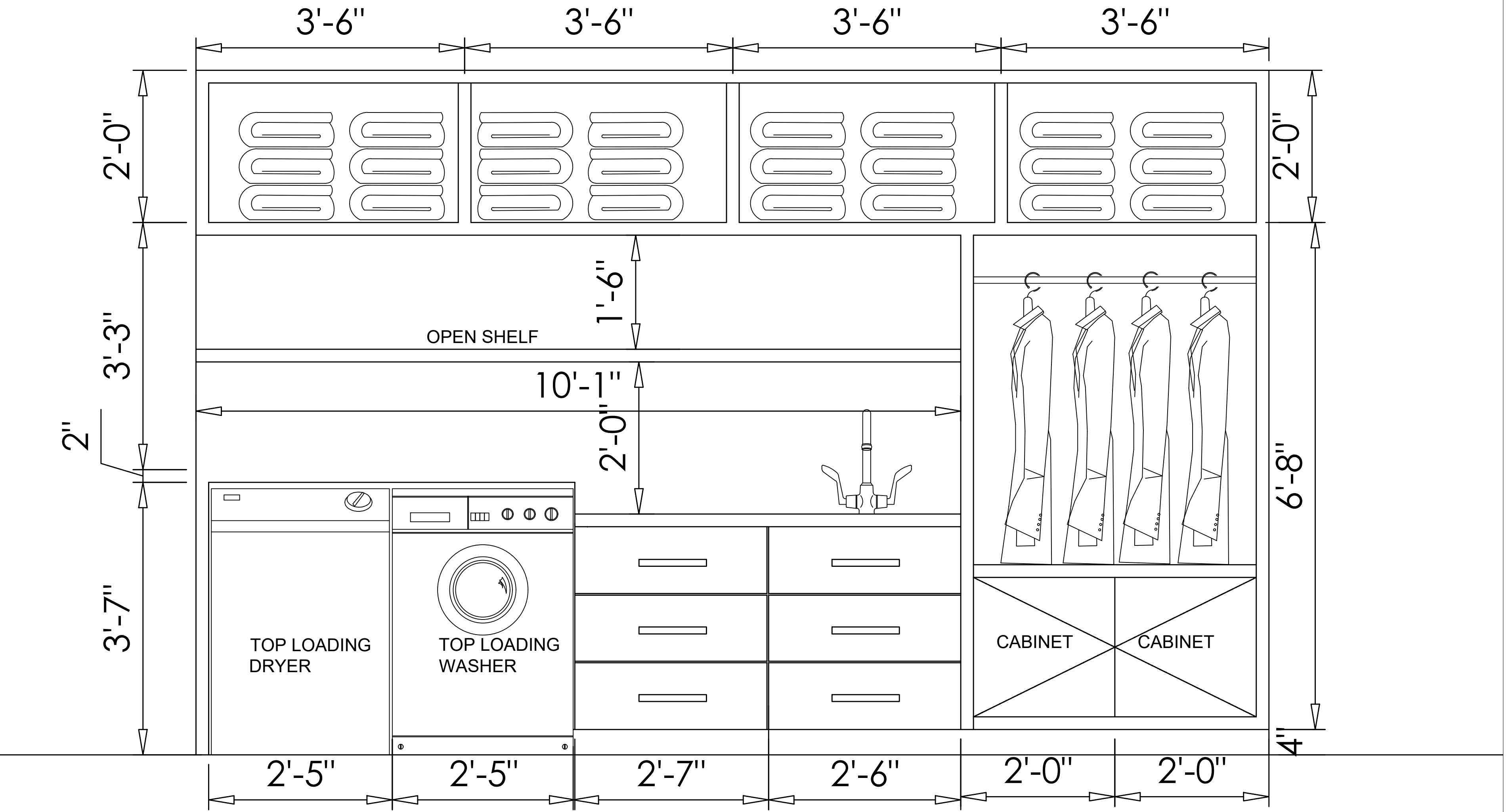
LAUNDRY ELEVATION SCALE : 1" = 1'
