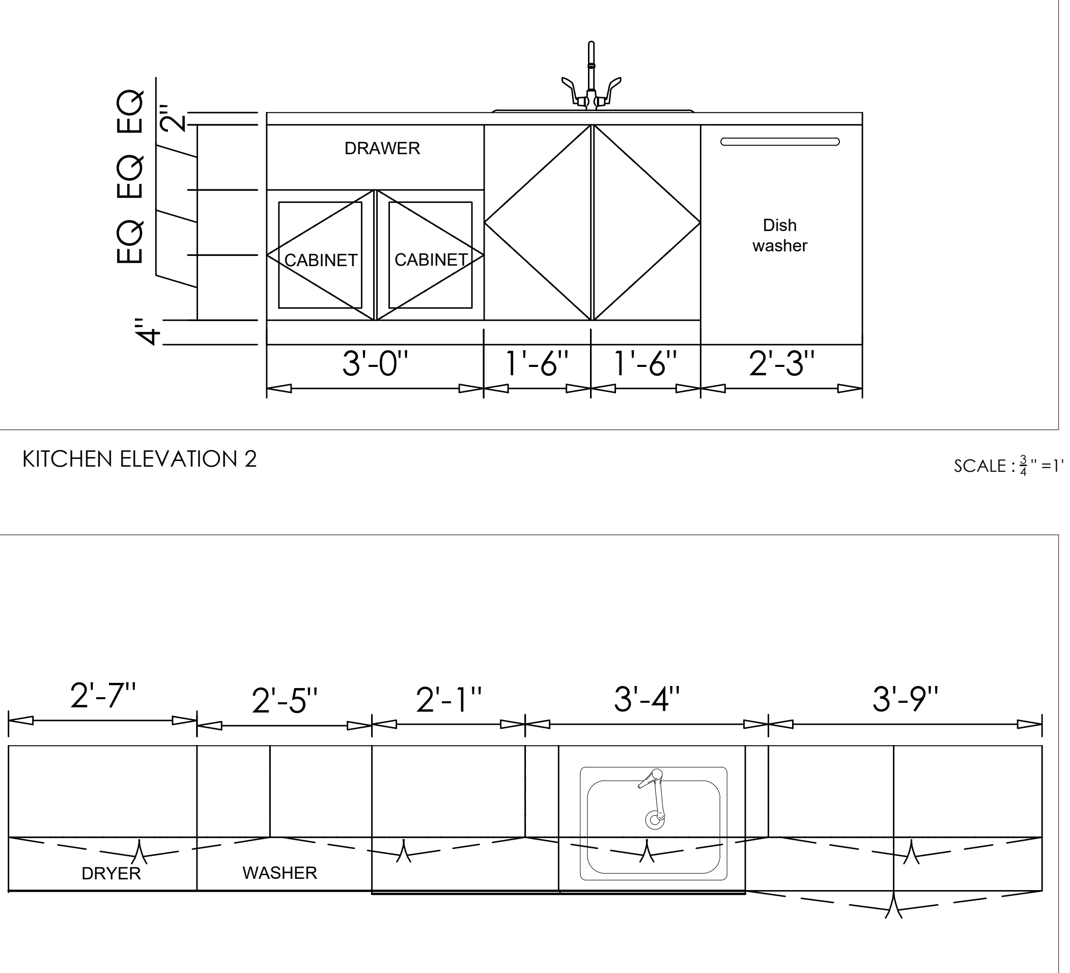
LAUNDRY PLAN SCALE : \frac{3}{4} " = 1'
