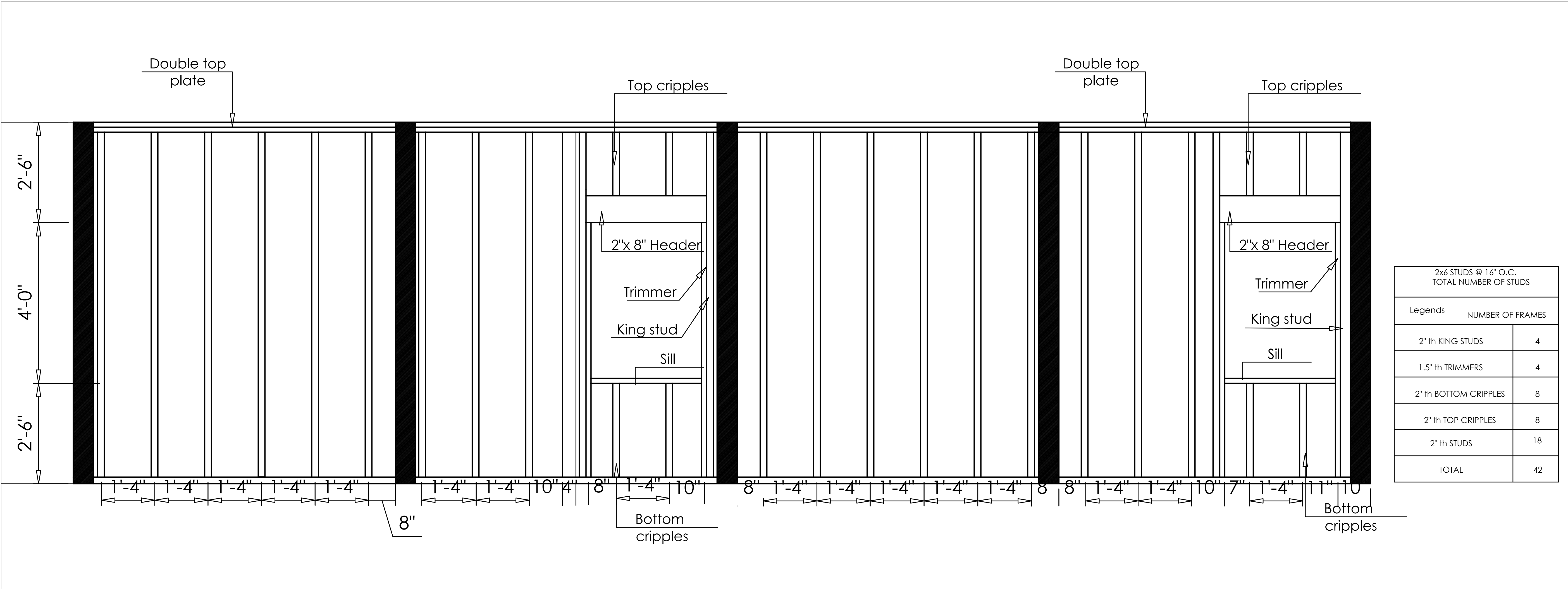
WALL CC FRAMING DETAILS
