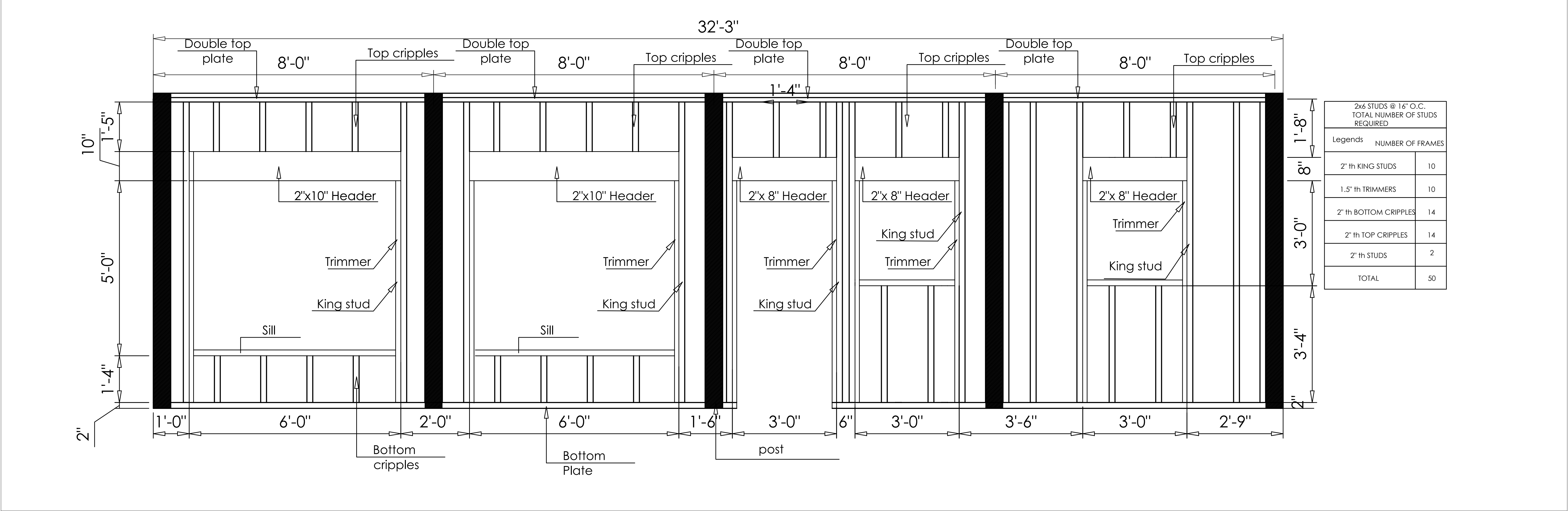
WALL AA FRAMING DETAILS
