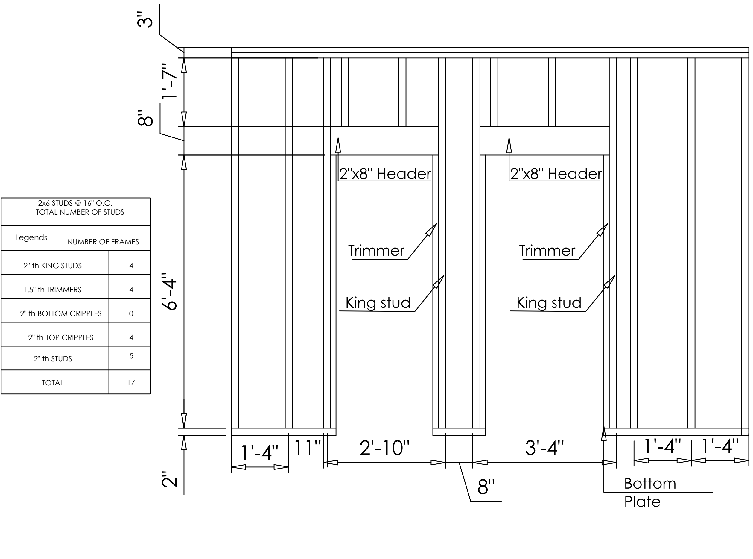
WALL H FRAMING DETAILS
