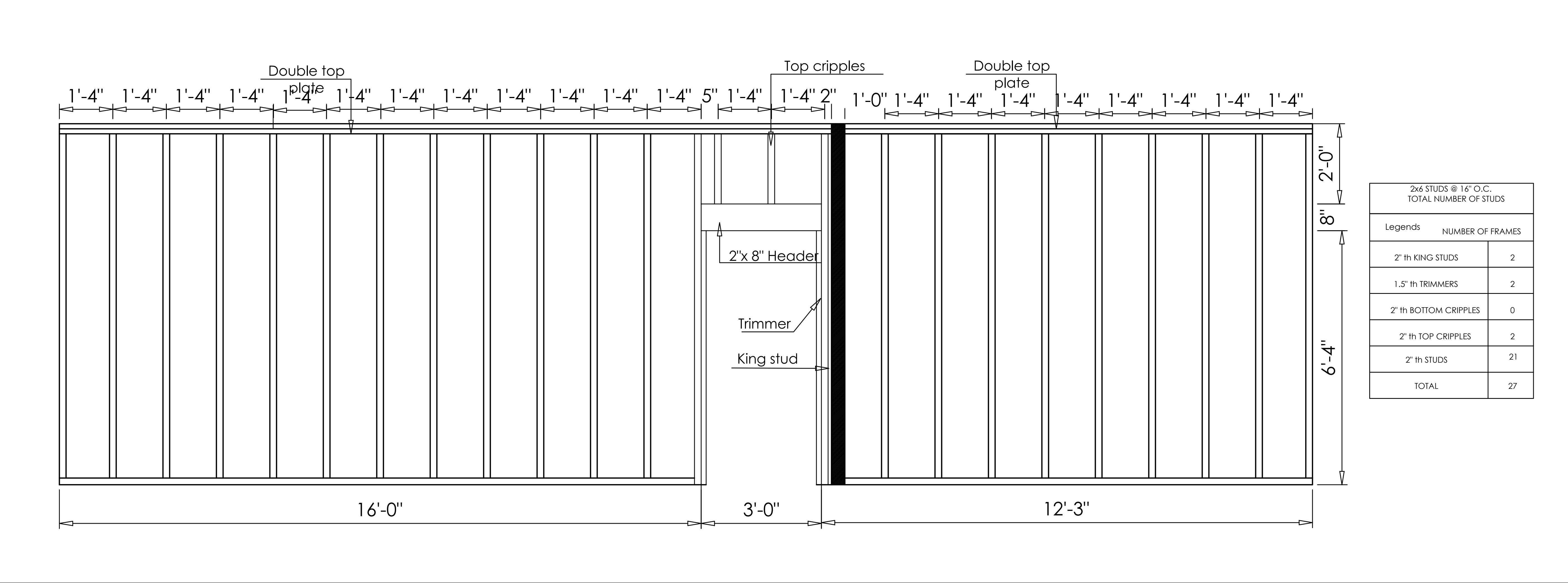
WALL EE FRAMING DETAILS
