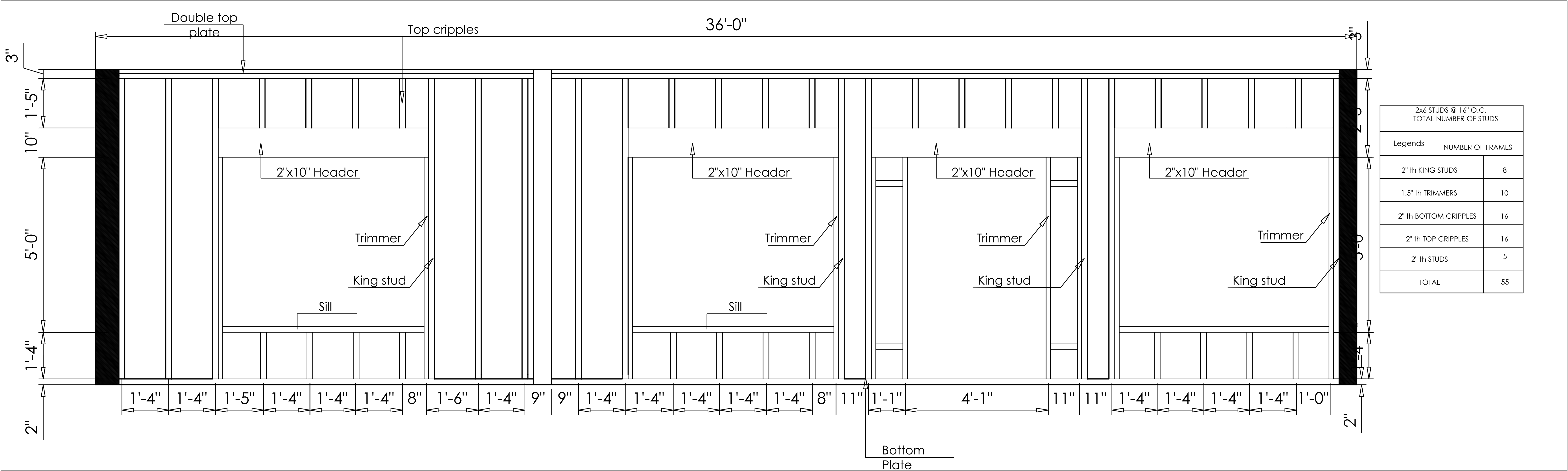
WALL BB FRAMING DETAILS
