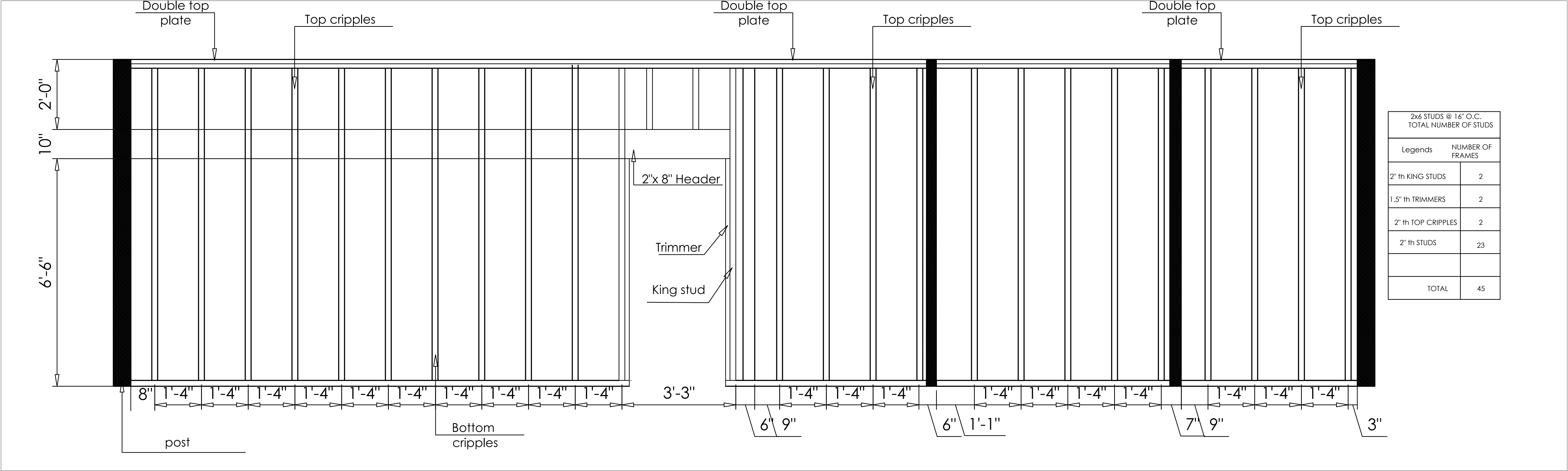
WALL DD FRAMING DETAILS
