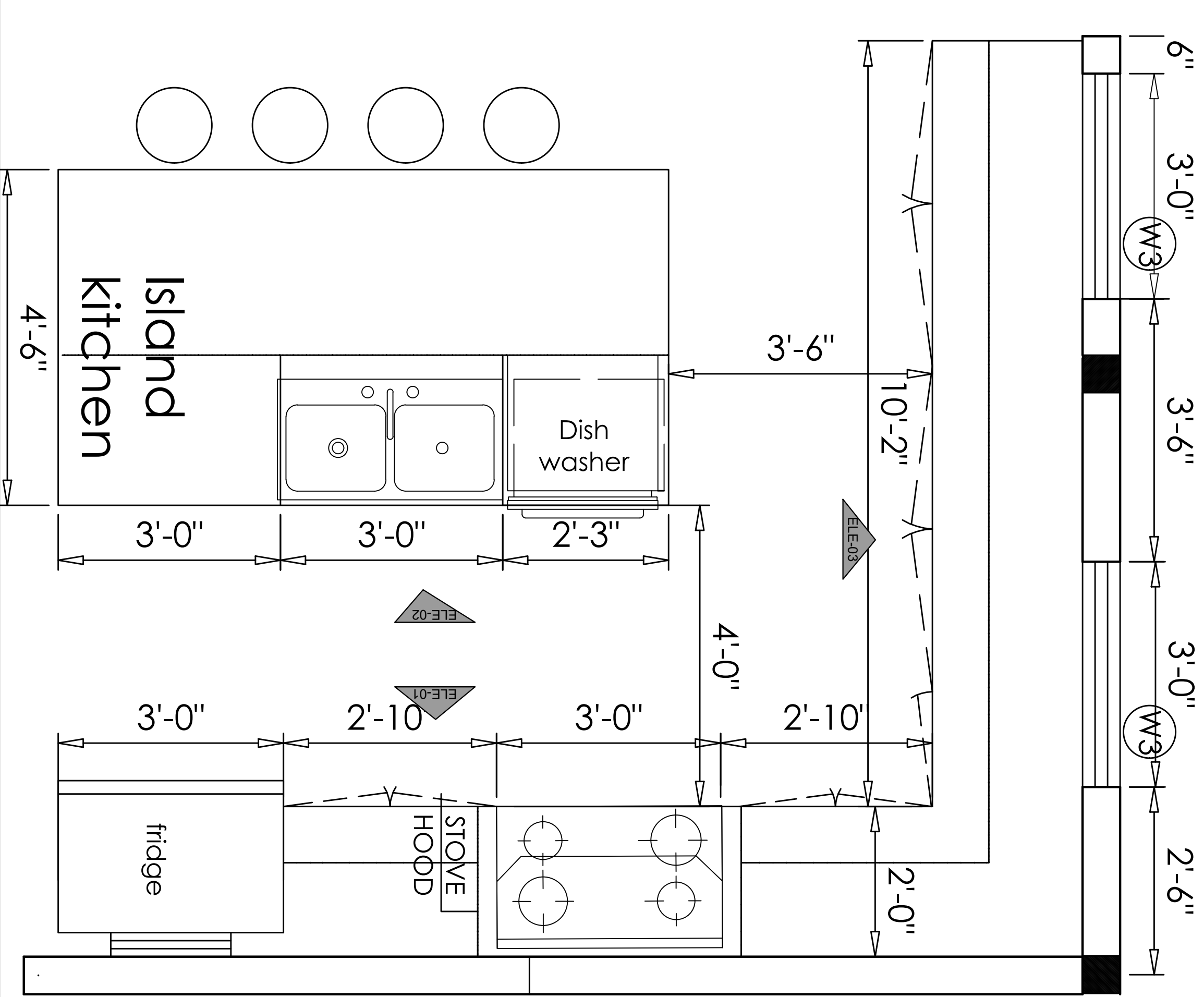
KITCHEN PLAN SCALE : \frac{3}{4} " = 1'
